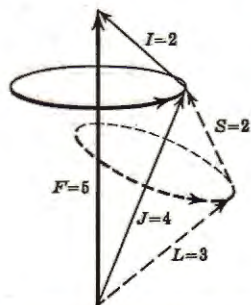
Fig. 70. Precession of the Angular Momentum Vectors about the Total Angular Momentum F for the Component F = 5 of a {}^6F_4 Term with I = 2 . The solid-line ellipse shows the precession of I and J about F . The dotted-line ellipse shows the much faster precession of L and S about J , taking place at the same time.
