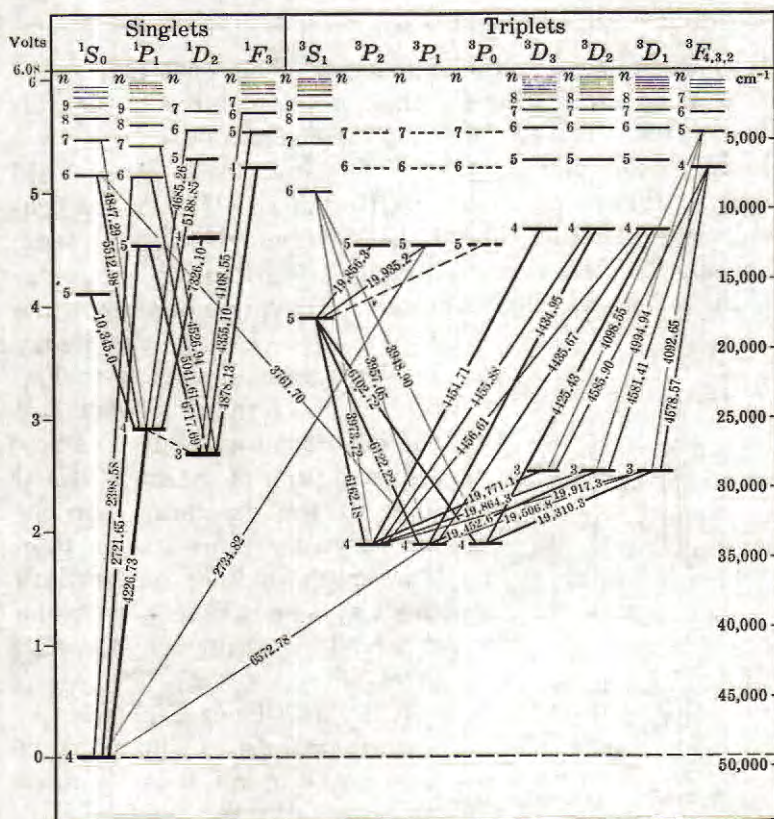
Fig. 32. Energy Level Diagram of Ca I [Grotrian (8)]. The diagram shows only the normal terms. (For the anomalous terms, see p. 164.) The n values are true principal quantum numbers. The transitions corresponding to spectrograms (a) to (c) in Fig. 31 are included, among others, in this figure.
