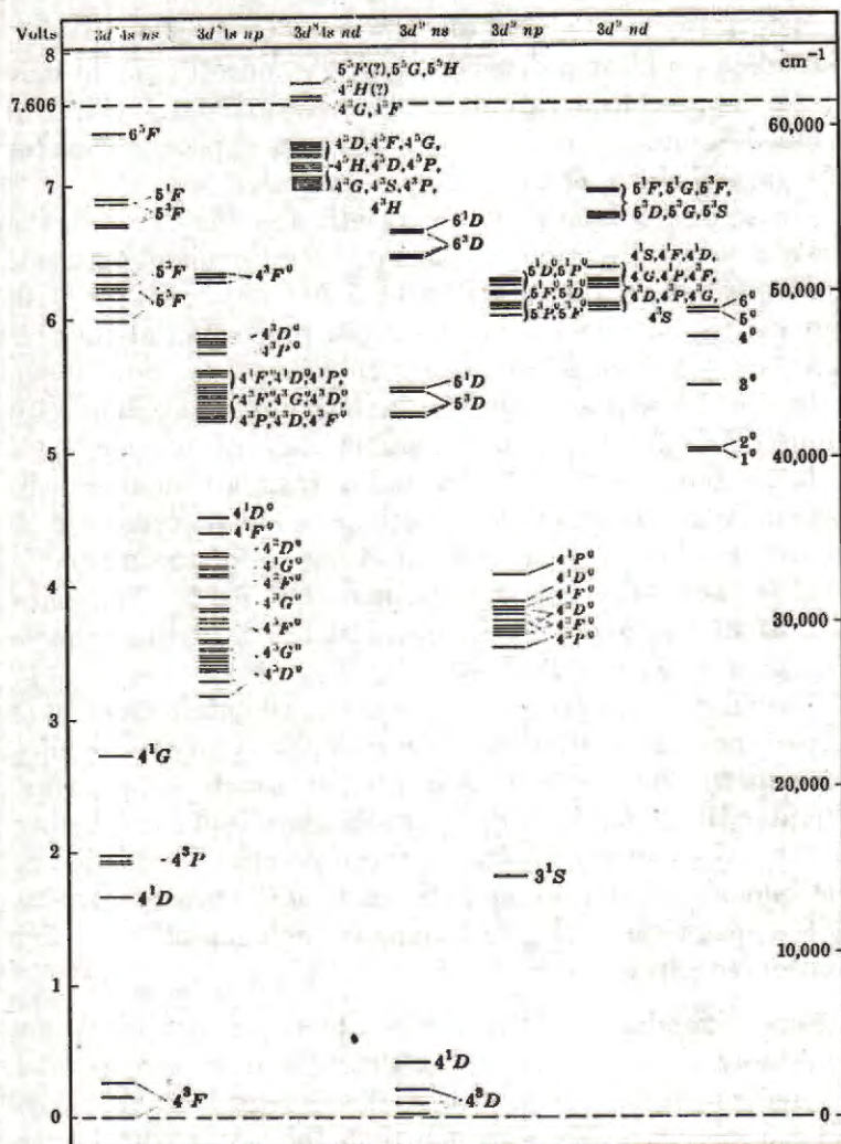
Fig. 76. Energy Level Diagram of Ni I [Russell (104)]. In general, the individual multiplet components are drawn separately, except for a few positions where too many terms nearly coincide with one another. Different terms of the same electron configuration (drawn above one another) do not usually go to the same limit. The lowest series limit (lowest ionization potential) is indicated by a dotted line.
