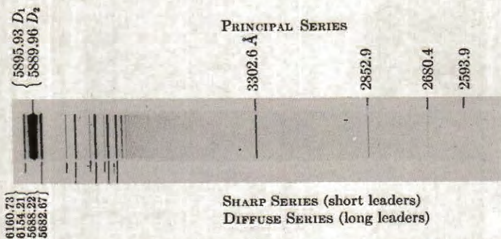
Fig. 3. Emission Spectrum of the Na Atom (Arc with One Na Electrode). Three series can be clearly recognized; one of them, the principal series, coincides with the absorption series of Fig. 2.
