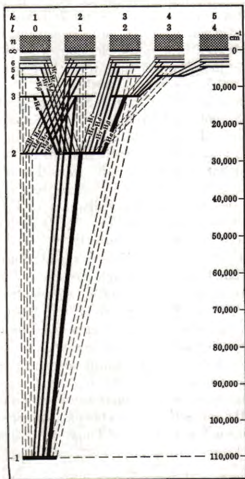
Fig. 13. Energy Level Diagram of the H Atom, Including Fine Structure [Grotrian (8)]. The Balmer series is indicated, as usual, with H_\alpha , H_\beta , H_\gamma , and so on. The broken lines refer to forbidden transitions.
