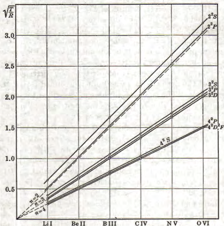
Fig. 26. Moseley Diagram of the Terms of Li-like Ions.
