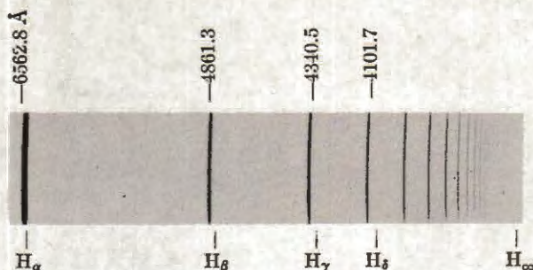
Fig. 1. Emission Spectrum of the Hydrogen Atom in the Visible and Near Ultraviolet Region [Balmer series, Herzberg (41)]. H_\infty gives the theoretical position of the series limit.
