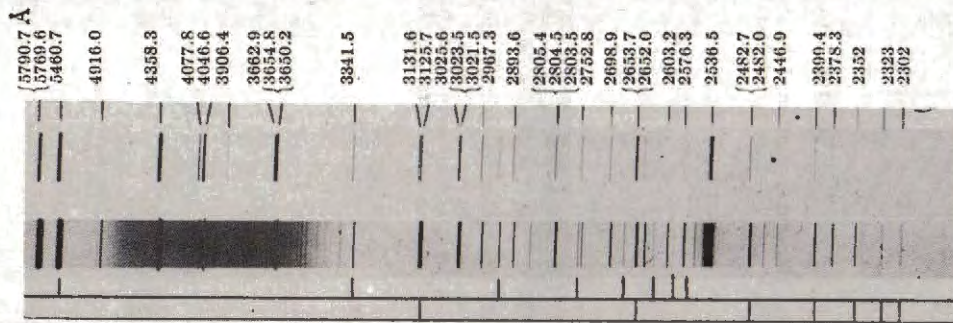
Fig. 5. Spectrum of a Mercury-Vapor Lamp. Two spectrograms with different exposure times are given, together with the wave lengths of most of the lines. This spectrum is often used as a comparison spectrum.
