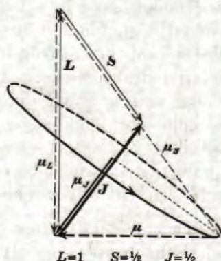
Fig. 48. Origin of the Magnetic Moment for a ^2P_{1/2} State. (Cf. Fig. 47.)
