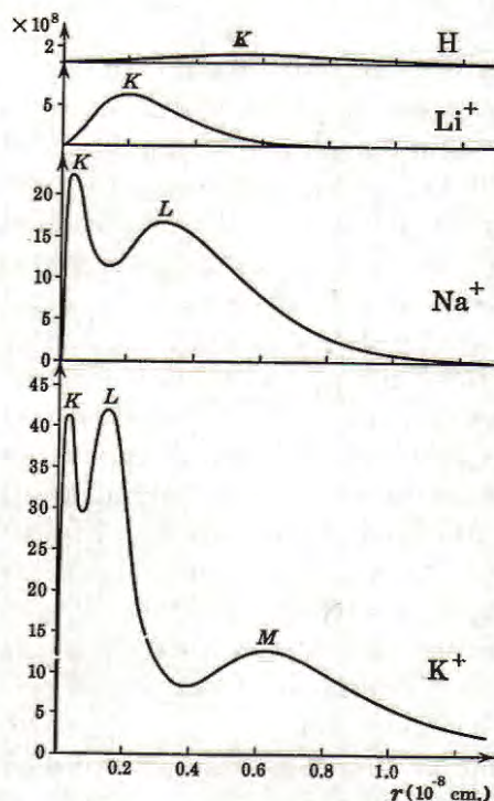
Fig. 54. Radial Charge Distribution for the Ground States of \text{H} , \text{Li}^+ , \text{Na}^+ , \text{K}^+ . The curves for \text{Na}^+ and \text{K}^+ are drawn according to the work of Hartree and his co-workers (62) and (63); the curve for \text{Li}^+ , according to Pauling and Goudsmit (9). All curves are drawn to the same scale.
