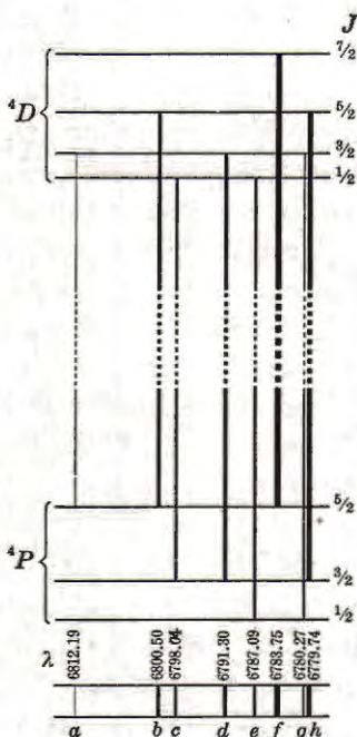
Fig. 34. 4P - 4D Transition for C^+ at 6800 Å. The relative separations of term and line components are drawn to scale from data given by Fowler and Selwyn (59).
