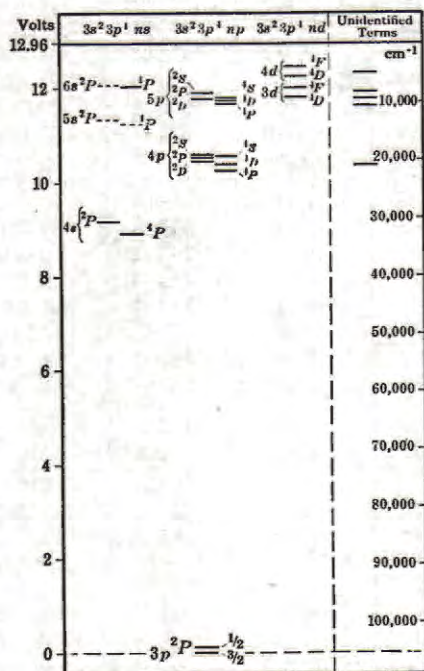
Fig. 74. Energy Level Diagram of Cl I [Kiess and de Bruin (103)]. Terms belonging to the same electron configuration are drawn under one another. Apart from the ground state, the different multiplet components are not drawn separately in the diagram.
