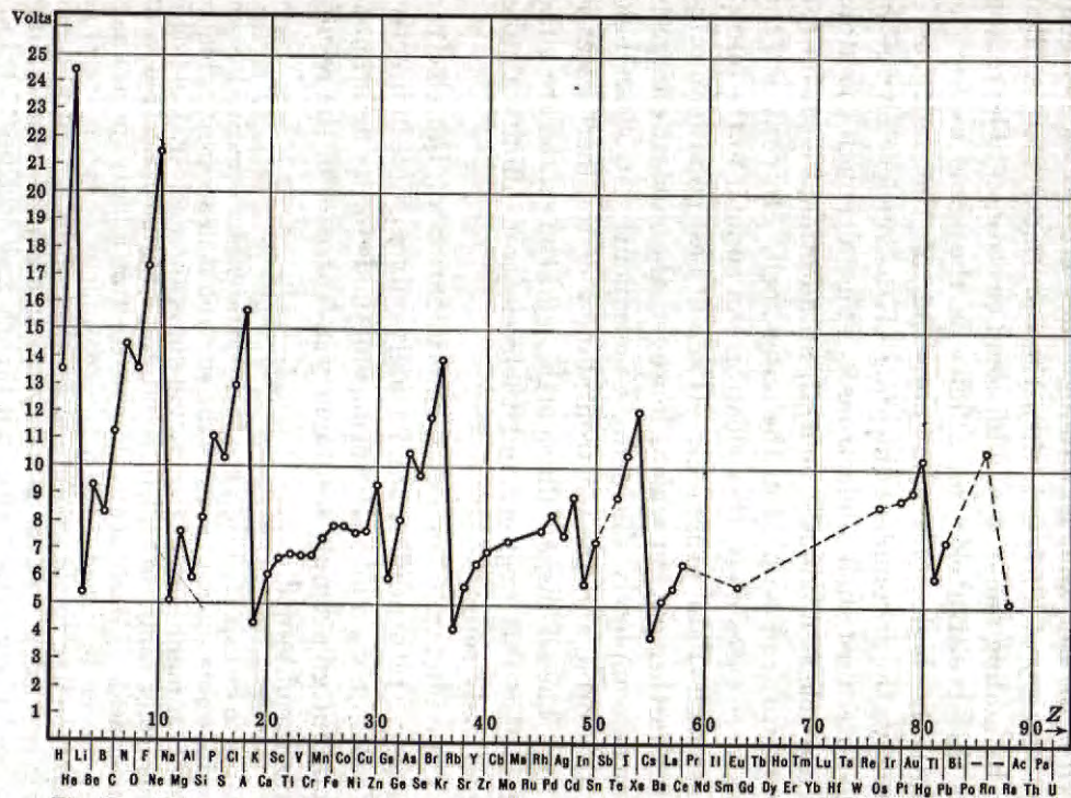
Fig. 78. Dependence of the Ionization Potential of the Neutral Atom on Atomic Number.
