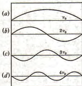
Fig. 16. Vibrations of a String: Fundamental and Overtones.
