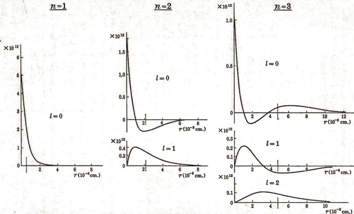
Fig. 18. Radial Part of Hydrogen Eigenfunctions for n = 1, 2, 3 . Abscissae give distance from nucleus in \text{\AA} ( 10^{-8} \text{ cm.} ); ordinates give normalized radial part of \psi . Curves with different values of n are drawn to different scales, as indicated.
