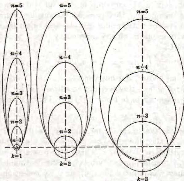
Fig. 10. Elliptical Bohr-Sommerfeld Orbits for the H Atom with k = 1, 2 , and 3 [from Grotrian (8)]. The positive nucleus is at the focus O of the ellipse. The energy difference between orbits with equal n but different k is very small. The smallest value of n for a given k is n = k . Same scale as in Fig. 9.
