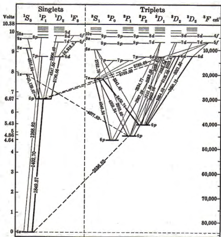
Fig. 75. Energy Level Diagram of Hg I [Grotrian (8)]. The wave lengths of the more intense Hg lines are given (cf. Fig. 5, p. 6). The symbols 6p, etc., written near each level, indicate the true principal quantum number and the l value of the emission electron.
