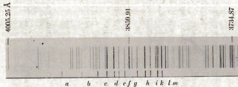
Fig. 6. Part of the Fe Arc Spectrum with Large Dispersion ( 2.7 \text{ Å/mm.} ). The multiplet indicated below is described fully in Chapter IV, section 4.
