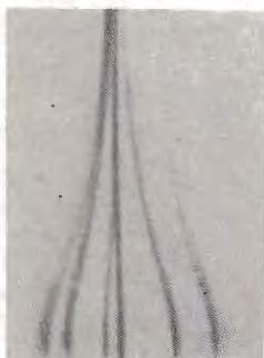
Fig. 50. Stark Effect Splitting of the Helium Line \lambda 4388 [after Foster (132)]. Above, the exposure was so made that only light polarized parallel to the field direction could reach the plate. Below, only light polarized perpendicular to the field could reach the plate. In each pattern the field increases from top to bottom.
