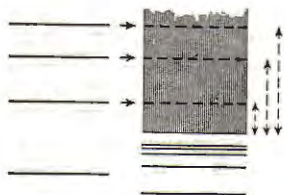
Fig. 64. Pre-ionization of the Terms Lying above the First Ionization Potential of an Atom or an Ion. To the left are shown the discrete terms that lie at the same height as the continuum which joins the series of terms drawn to the right.
