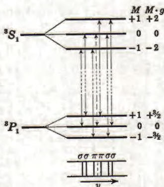
Fig. 46. Anomalous Zeeman Splitting of a ^3S_1 \rightarrow ^3P_1 Transition. [Cf. Fig. 39 (c), p. 97.] According to the selection rule (II, 13), the transition M = 0 \rightarrow M = 0 is forbidden, since at the same time \Delta J = 0 . This transition is indicated by a dotted line.
