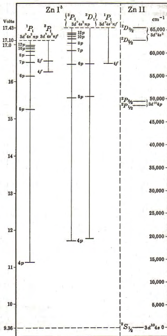
Fig. 62. Energy Level Diagram of Zn I b [Beutler and Guggenheimer (80)]. A part of the energy level diagram of Zn II is drawn to the right. The scale of volts to the left starts from the ground state of Zn as zero. The cm -1 scale to the right starts from the ground state of Zn + as zero.
