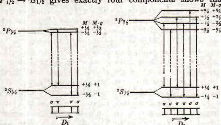
Fig. 45. Anomalous Zeeman Effect of the Sodium D Lines, ^2P_{1/2} \rightarrow ^2S_{1/2} and ^2P_{3/2} \rightarrow ^2S_{1/2} . [Cf. Fig. 39 (b), p. 97.] The components designated by \sigma have \Delta M = \pm 1 ; those designated by \pi have \Delta M = 0 . It should be noted that, contrary to Fig. 44, arrows indicating transitions with equal \Delta M no longer have the same length, because of the difference in the splitting in the upper and lower states.
