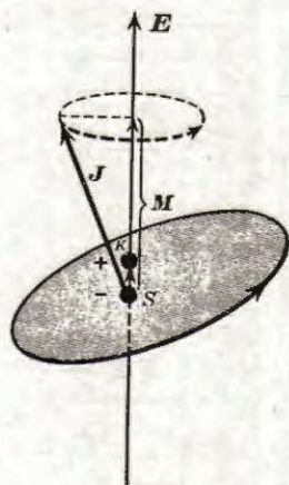
Fig. 51. Production of an Electric Dipole Moment in an Electric Field (Stark Effect) and Precession of J about the Field Direction. The shaded surface represents the orbital plane of the atom. The angular momentum vector is perpendicular to that plane.
