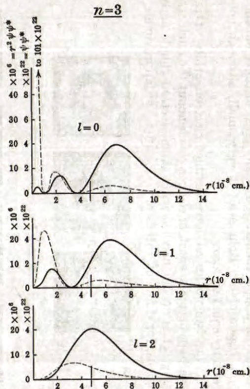
Fig. 20. Probability Density Distribution of the Electron for n=1, 2, 3 for the H Atom Plotted as a Function of the Distance r . Dotted curves represent \psi\psi^* ; solid curves, r^2\psi\psi^* . All curves are drawn to the same scale (outer scale for r^2\psi\psi^* ; inner scale for \psi\psi^* ). \psi\psi^* dr gives the probability of finding the electron in a volume element dr (the dimensions of \psi\psi^* are therefore \text{cm}^{-3} ); r^2\psi\psi^* dr gives the probability of finding the electron in the spherical shell of thickness dr at a distance r from the mid-point.
