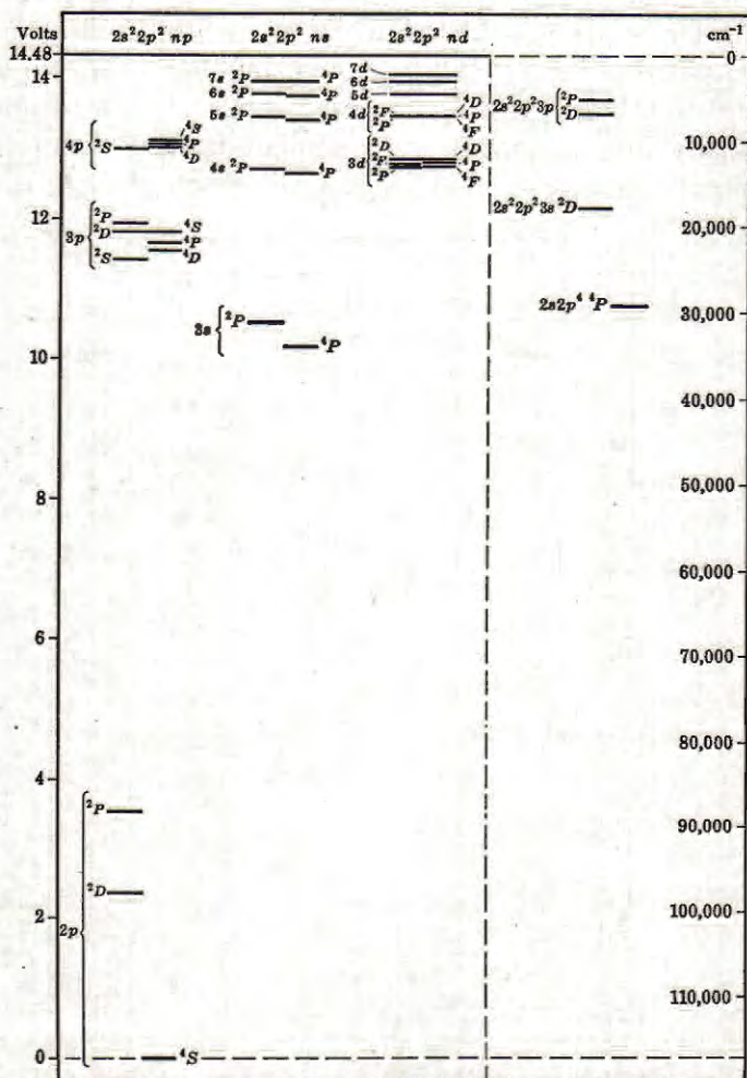
Fig. 56. Energy Level Diagram for N I.
