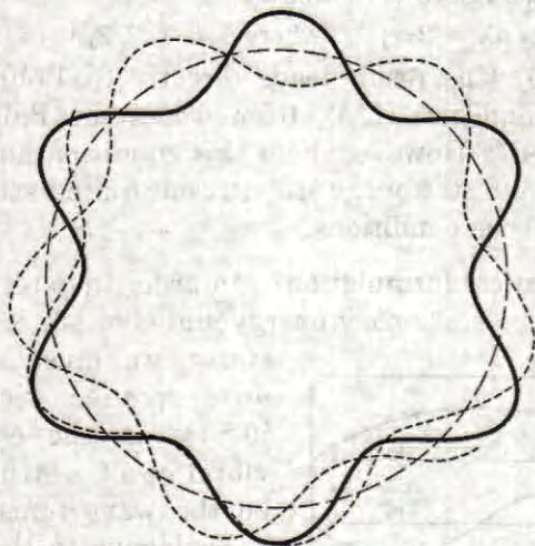
Fig. 15. De Broglie Waves for the Circular Orbits of an Electron about the Nucleus of an Atom (Qualitative). Solid line represents a stationary state (standing wave); dotted line, a quantum-theoretically impossible state (waves destroyed by interference).
