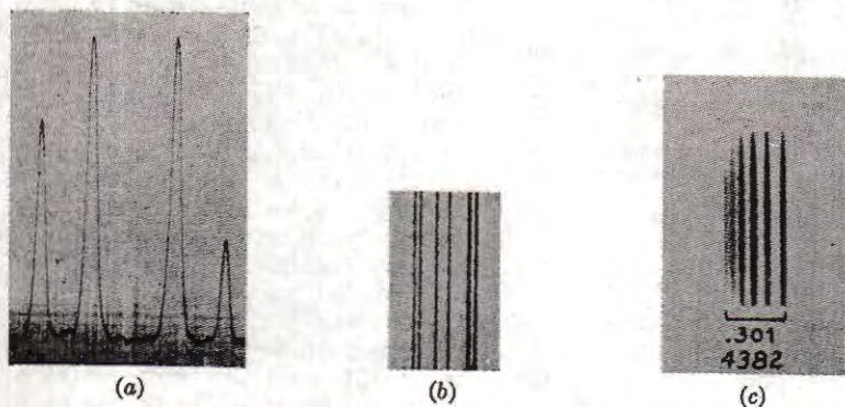
Fig. 67. Hyperfine Structure of Three Spectral Lines. (a) Photogram of the "line" 4122 Å of Bi I, with 4 components. Total splitting 0.44 Å [Zeeman, Back, and Goudsmit (83)]. (b) Spectrogram of the "line" 5270 Å of Bi II, with 6 components. Total splitting 1.37 Å [Fisher and Goudsmit (84)]. (c) Spectrogram of the "line" 4382 Å of Pr II, with 6 components. Total splitting 0.30 Å [White (85)].
