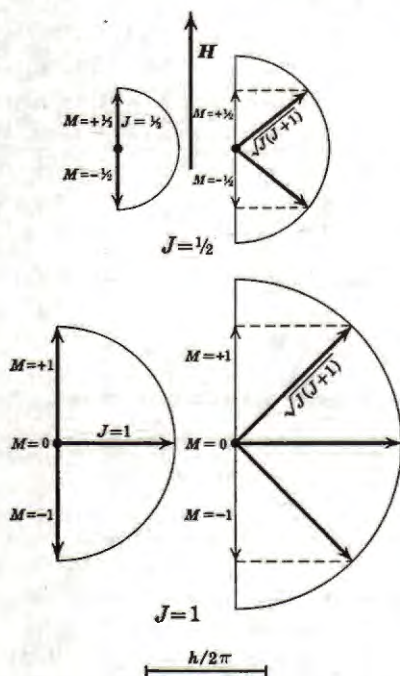
Fig. 43. Space Quantization for J = \frac{1}{2} and J = 1 . To the left is the naive representation (see Fig. 41) taking the magnitude of the total angular momentum equal to J(h/2\pi) . To the right is the exact representation taking the magnitude equal to \sqrt{J(J+1)} h/2\pi .
