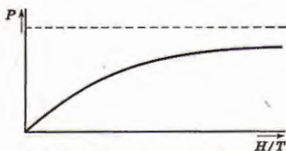
Fig. 77. Dependence of Magnetization P on Field Strength and Absolute Temperature, H/T (Langevin). The dotted horizontal line corresponds to paramagnetic saturation.
