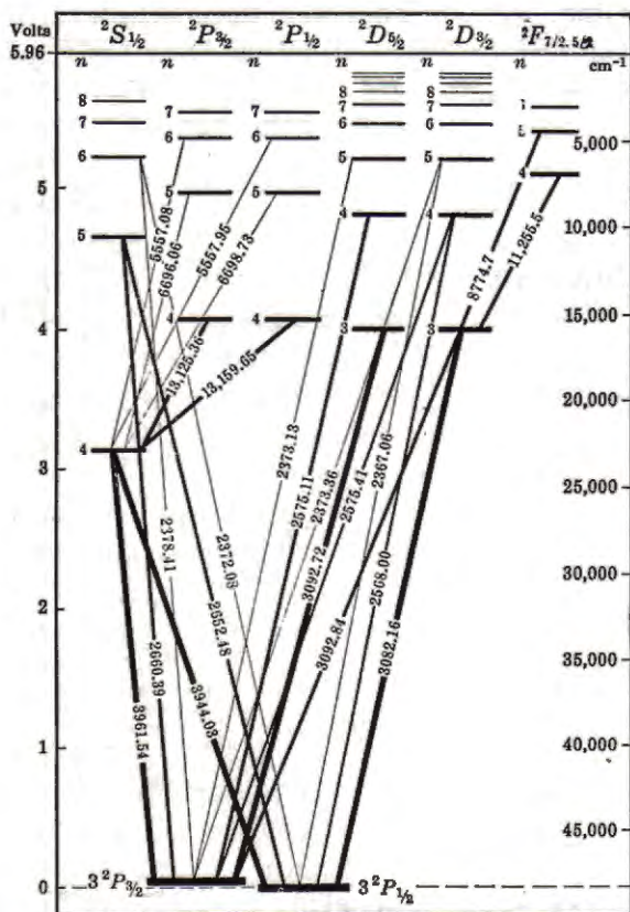
Fig. 73. Energy Level Diagram of Al I [Grotrian (8)]. n is the true principal quantum number of the emission electron. Only the normal doublet terms are indicated, all of which go to the same limit. Series of anomalous terms (doublets and quartets) have been observed by Paschen (64).
