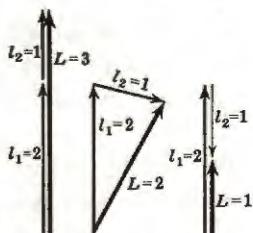
Fig. 35. Addition of l_1 and l_2 to Give a Resultant Orbital Angular Momentum L for l_1 = 2 , l_2 = 1 , and L = 3, 2, 1 .
