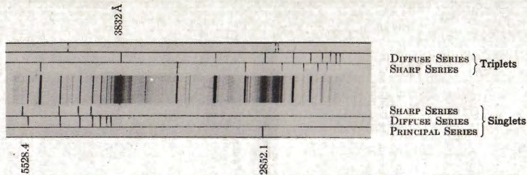
Fig. 4. Arc Spectrum of Magnesium. The different series of the neutral Mg atom are indicated above and below. See Chapter I, section 6. The spectral lines indicated with dotted lines do not belong to the normal series. The few weaker unmarked lines in the spectrogram are lines of Mg^+ and impurities.
