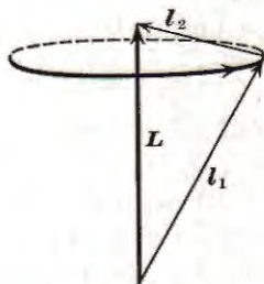
Fig. 36. Precession of l_1 and l_2 about the Resultant L . Replacing l_1 , l_2 , and L by L , S , and J gives a picture of the precession of L and S about J . (See p. 90.)
