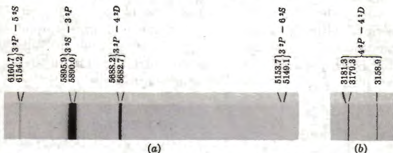
Fig. 29. Examples of Line Doublets. (a) Some Na doublets (part of the Na emission spectrum reproduced in Fig. 3, taken with larger dispersion). (b) Compound doublet of \text{Ca}^+ . True principal quantum numbers are used to designate the terms.
