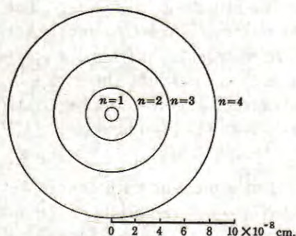
Fig. 9. Circular Bohr Orbits for the H Atom ( n = 1 to n = 4 ).
