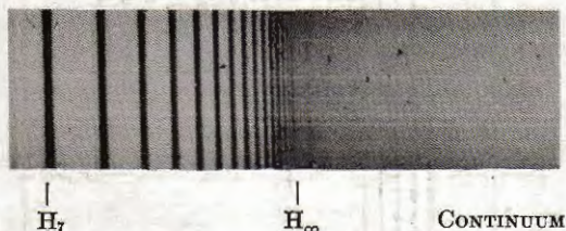
Fig. 11. Higher Members of the Balmer Series of the H Atom (in Emission) Starting from the Seventh Line and Showing the Continuum [Herzberg (41)]. H_\infty gives the theoretical position of the series limit. The photograph was more strongly exposed than Fig. 1, and consequently some weak molecular lines not belonging to the Balmer series are also present—for example, one in the neighborhood of the position of H_\infty .
