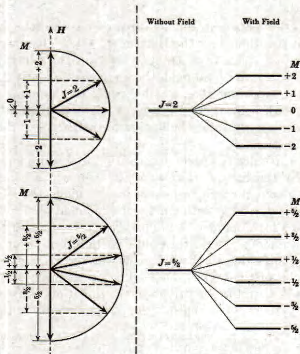
Fig. 41. Space Quantization of the Total Angular Momentum J in a Magnetic Field H for J = 2 and J = \frac{5}{2} . To the left are the possible orientations to the magnetic field. To the right, in an energy level diagram, the corresponding energy values are indicated.
